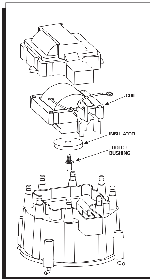
Figure 1 Installing the MSD GM HEI Coil.
